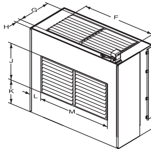
(1) DETAIL A SHOWS THE AIRSIDE ECONOMIZER WITH ALL DAMPER CONFIGURATIONS CURRENTLY AVAILABLE AND ALL OPENING DIMENSIONS (NECESSARY FOR DUCT WORK).
